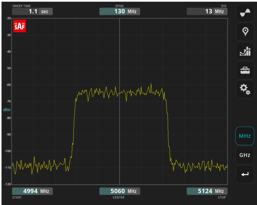
The main window of Spectrum Manager started in REALTIME mode.
